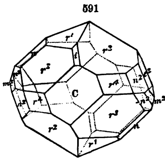
Brewster.
